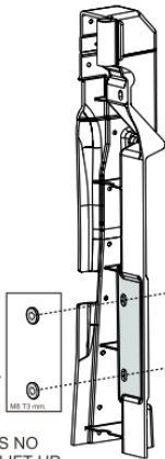
SCREW M8x30 L x4 WASHER M8x1.2 OD30 M x4 WASHER M8 THICKNESS 3 mm. P x4
