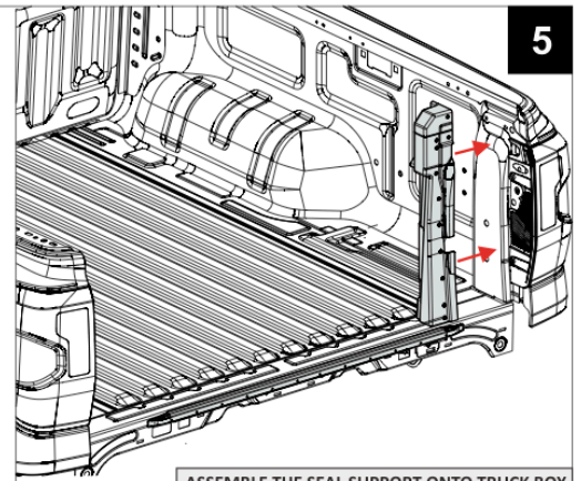
ASSEMBLE THE SEAL SUPPORT ONTO TRUCK BOX
